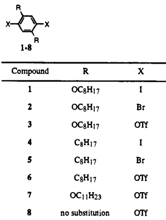
Figure 1. Structures of the organohalides and triflates for the Stille coupling reactions.
