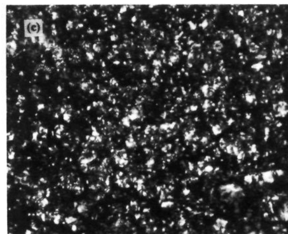
Figure 6. Typical Schleiern textures under a polarizing microscope, indicating a nematic liquid crystalline phase: (a) polymer 1 ( n = 7 ), 90 °C, 100 ×; (b) polymer 3 ( n = 8 ), 173 °C, 100 ×; (c) polymer 5 ( n = 8 ), 95 °C, 100 ×. All parts were reproduced at 80% of the original size.
